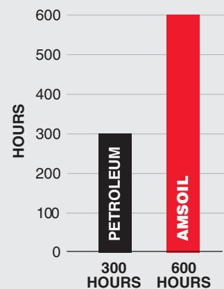
High Temperature Tests Ford MERCON® V required oxidation test (ABOT)
